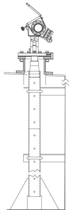
Stillwell installation Radar waves guided to tank bottom, avoiding unwanted reflections
