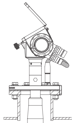
Standard installation Mounted on a small deck socket / trunk
